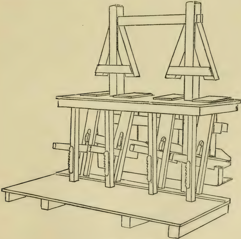
Raisin Lever Press.
